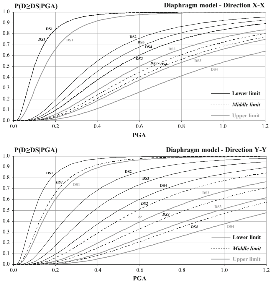
Fig. 16 Fragility curves for the fully strengthened building model (rigid diaphragm)
