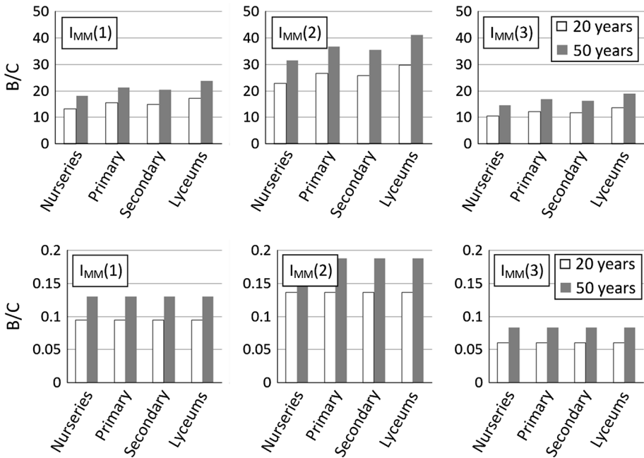
Fig. 22 Benefit/cost ratios for masonry buildings using the lower bound of fragility curves, assuming full diaphragm action after retrofit, with ( top ) and without ( bottom ) taking into account the statistical value of human life, for the three hazard relationships ( I_{MM} )
