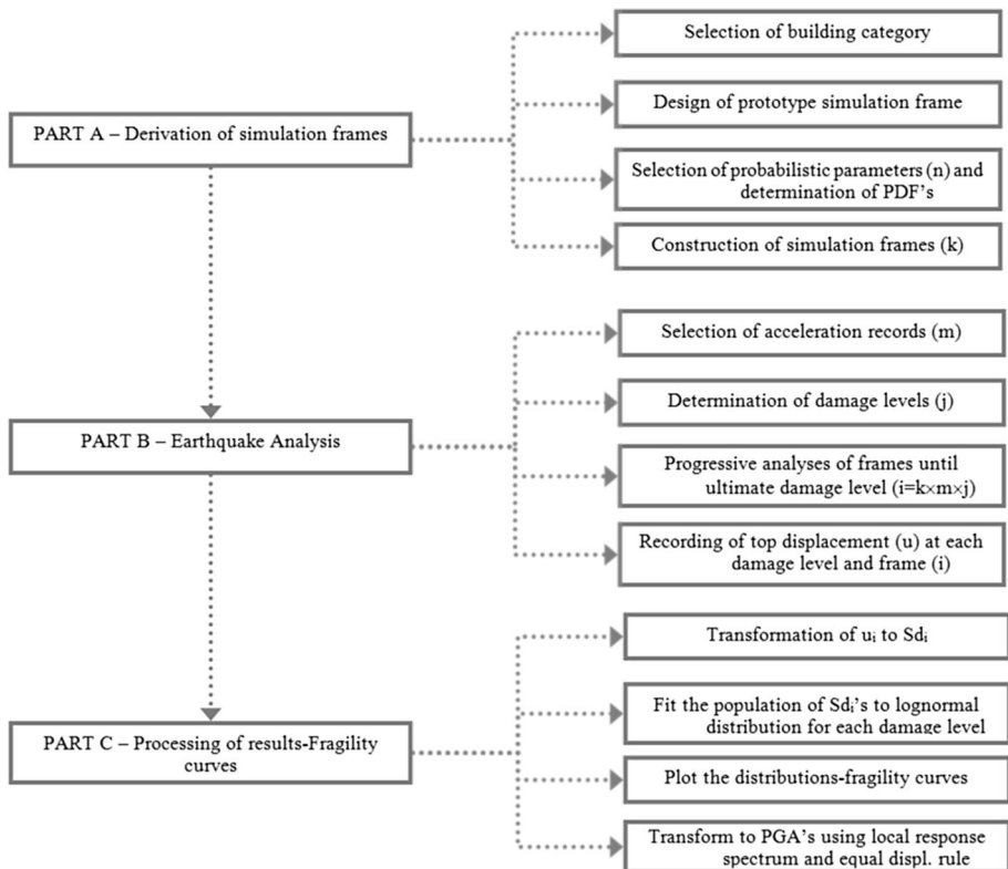
Fig. 5 Framework for the derivation of PGA fragility curves
