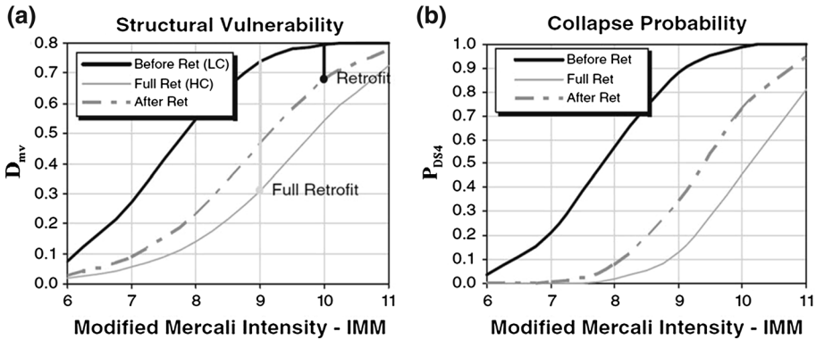
Fig. 18 Efficiency of seismic strengthening. Reduction of structural vulnerability after full or intermediate retrofit in terms of a Mean Damage Factor ( D_{MV} ) and b Collapse Probability ( P_{DSi} )
