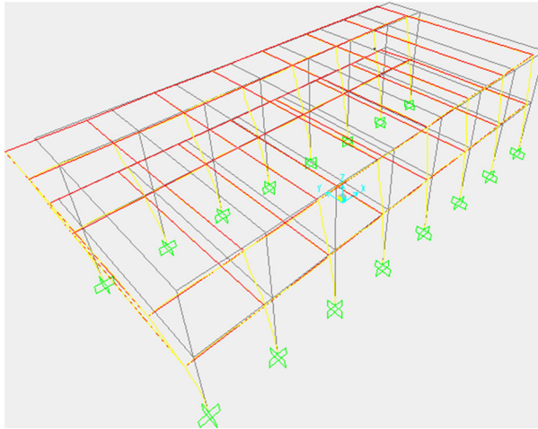
Fig. 4 Structural model and fundamental mode shape of R/C building
