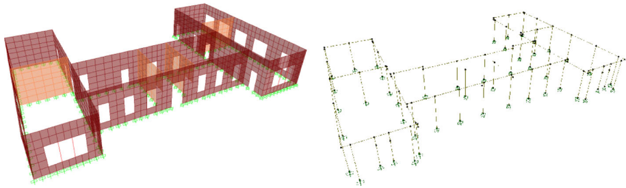
Fig. 10 Finite element modelling: shell ( left ) and equivalent frame
