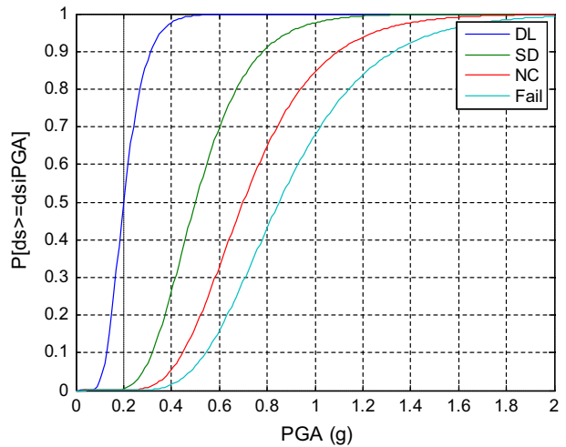
Fig. 8 PGA fragility curves for the strengthened R/C school building
