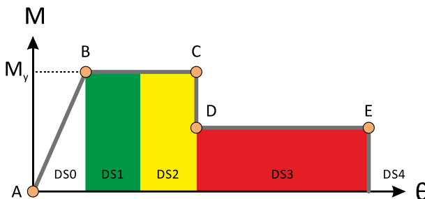
Fig. 12 Definition of damage states
