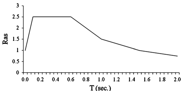
Fig. 6 Normalised response spectrum based on the local microzonation study
