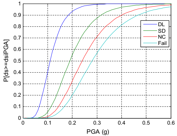
Fig. 7 PGA fragility curves for the pristine R/C school building
