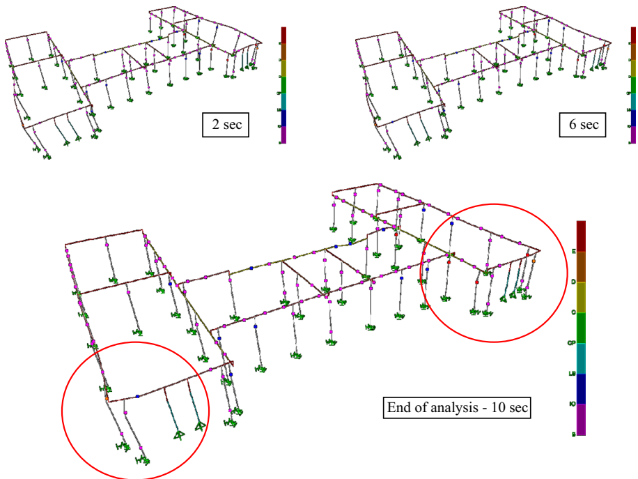
Fig. 14 Damage sequence and localisation at corners
