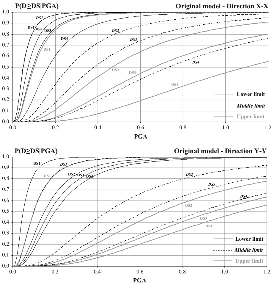
Fig. 15 Fragility curves for the pristine building model
